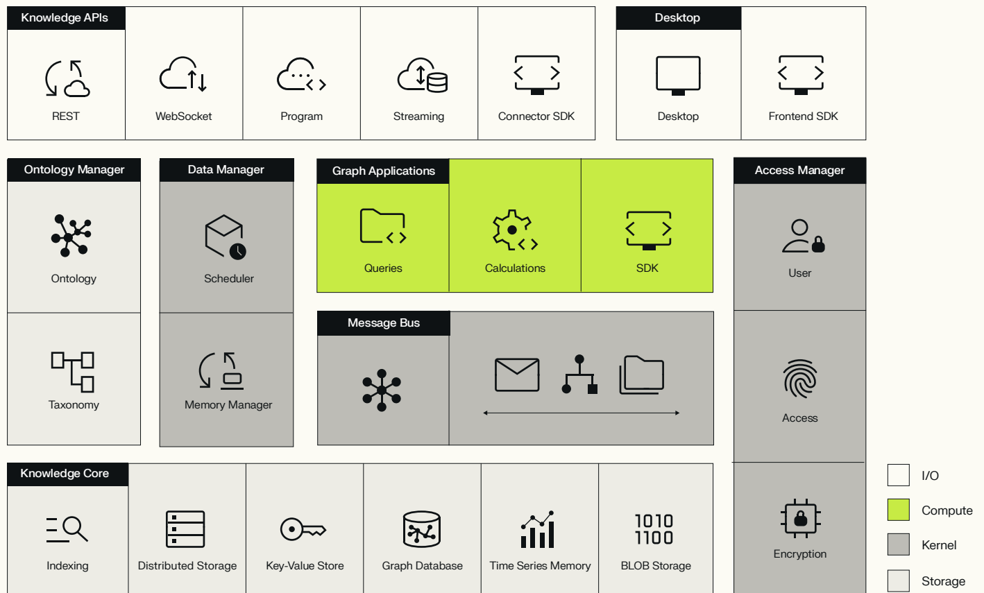
Functional architecture of Bardioc
